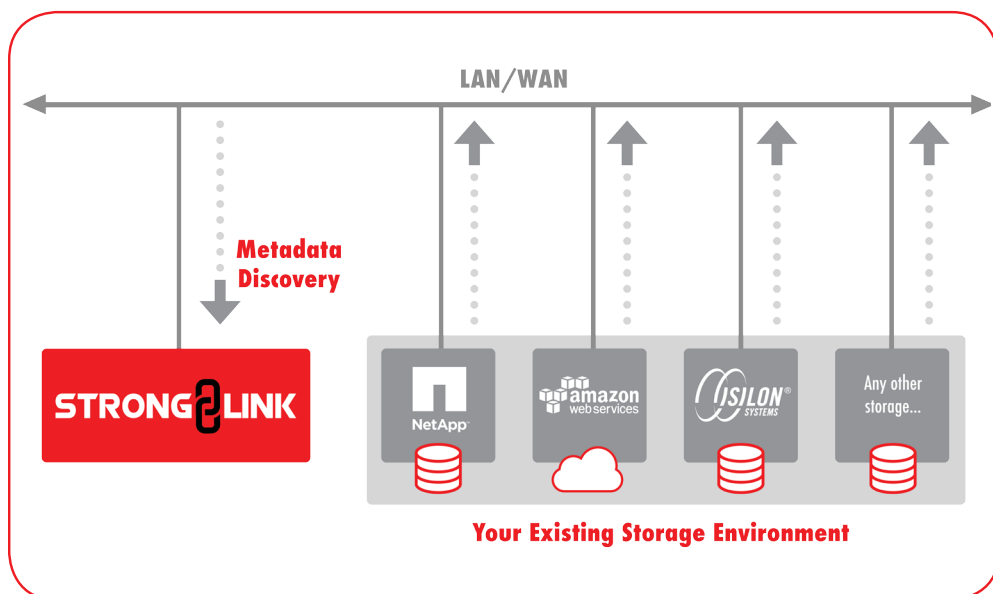
StrongLink harvests multiple types of file and system metadata from any storage type or file system, which can be used for search, policy-based data migrations, and much more, with a global view across all storage silos.
